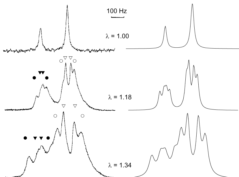
Fig. 2. 2 H NMR spectra of PBD probe chains diffusing through the PB network observed for various extension ratio \lambda . Left side: experimental spectra; right side: calculated spectra. The doublets are assigned as following: (a) cis units—CD 2 component (▽), (b) cis units—CD component (▼), (c) trans units—CD 2 component (○) and (d) trans units—CD component (●).
